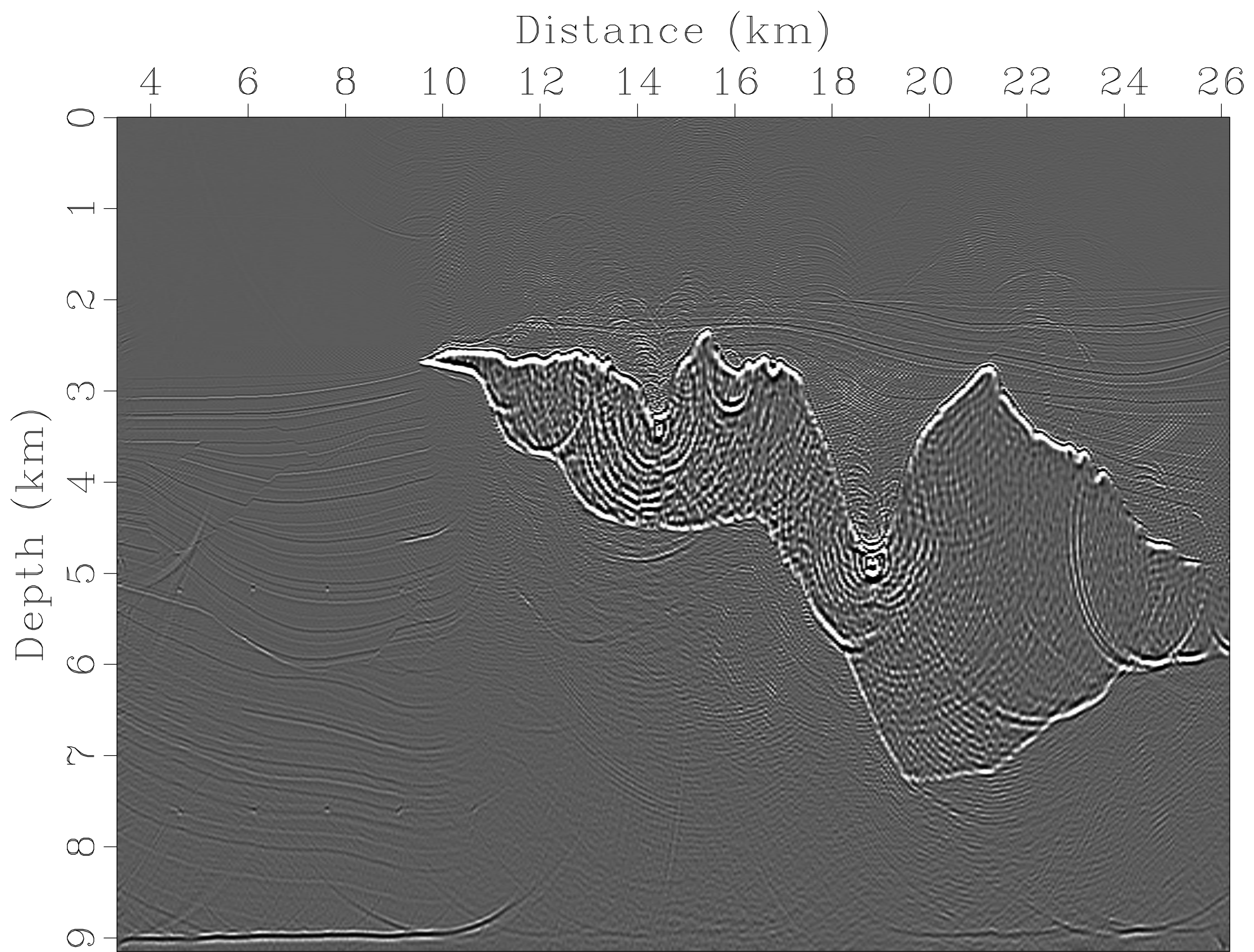
Zero-Offset Migration
