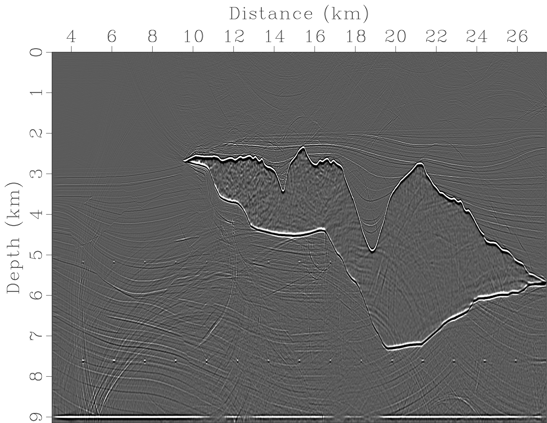
Zero-Offset Migration
