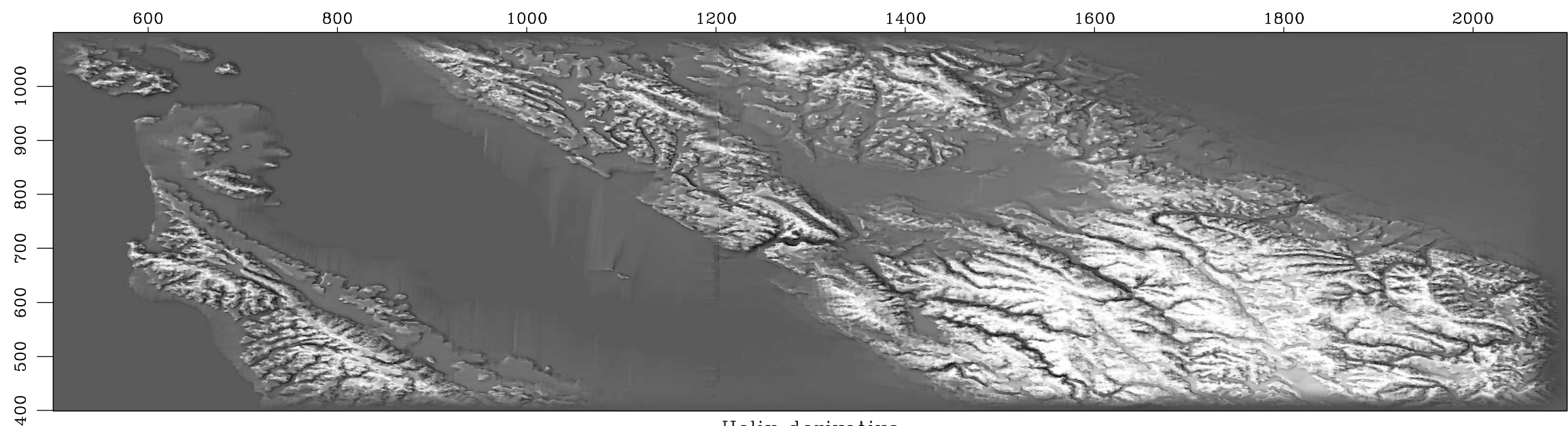
Helix derivative
