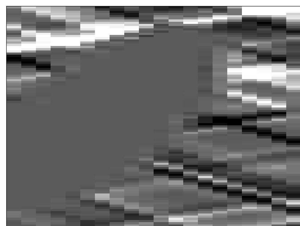
singlescale, iter=1
