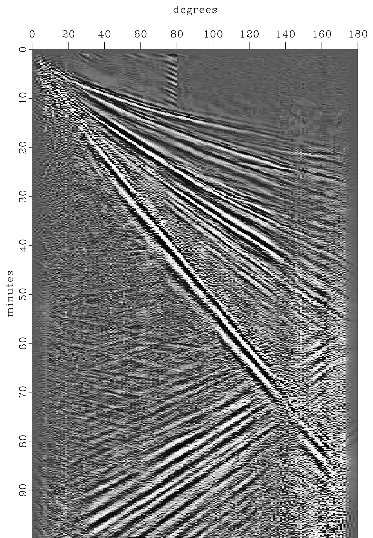
epsilon=2
