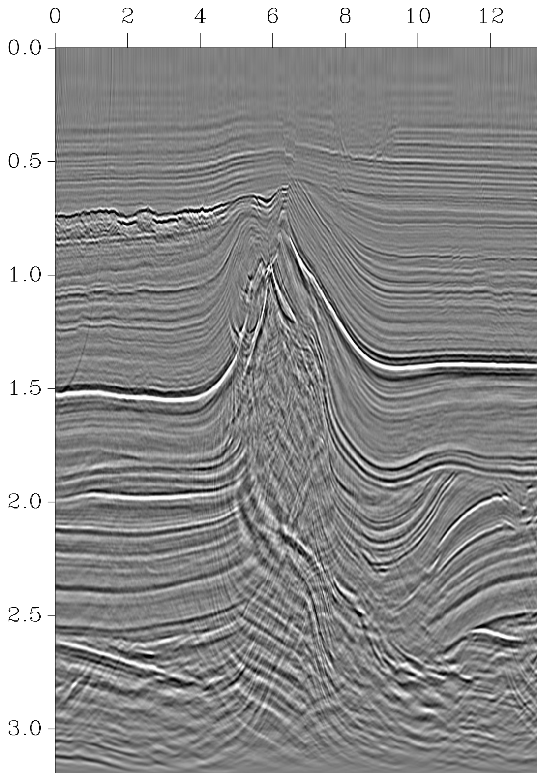
Prestack time migration
