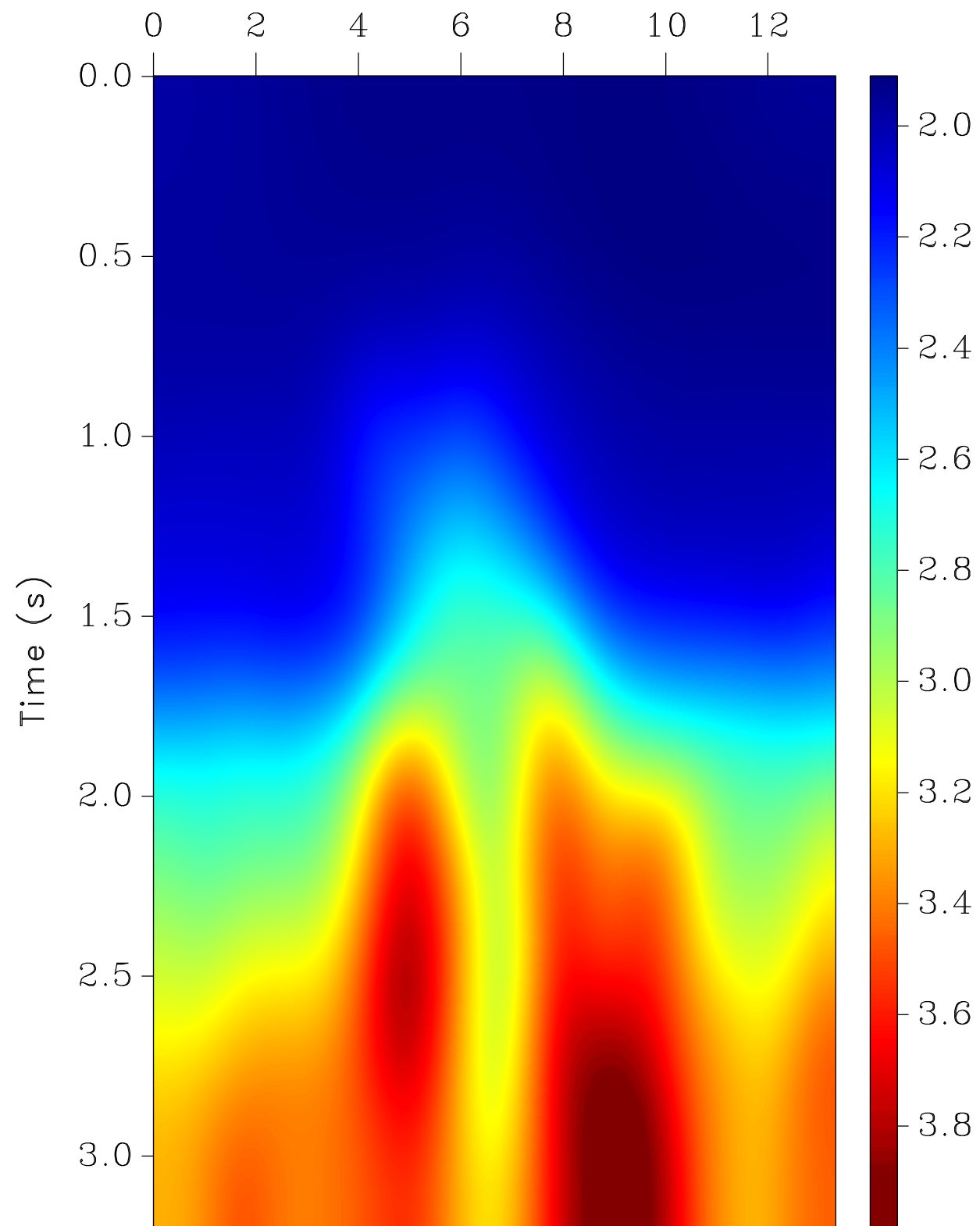
Time migration velocity
