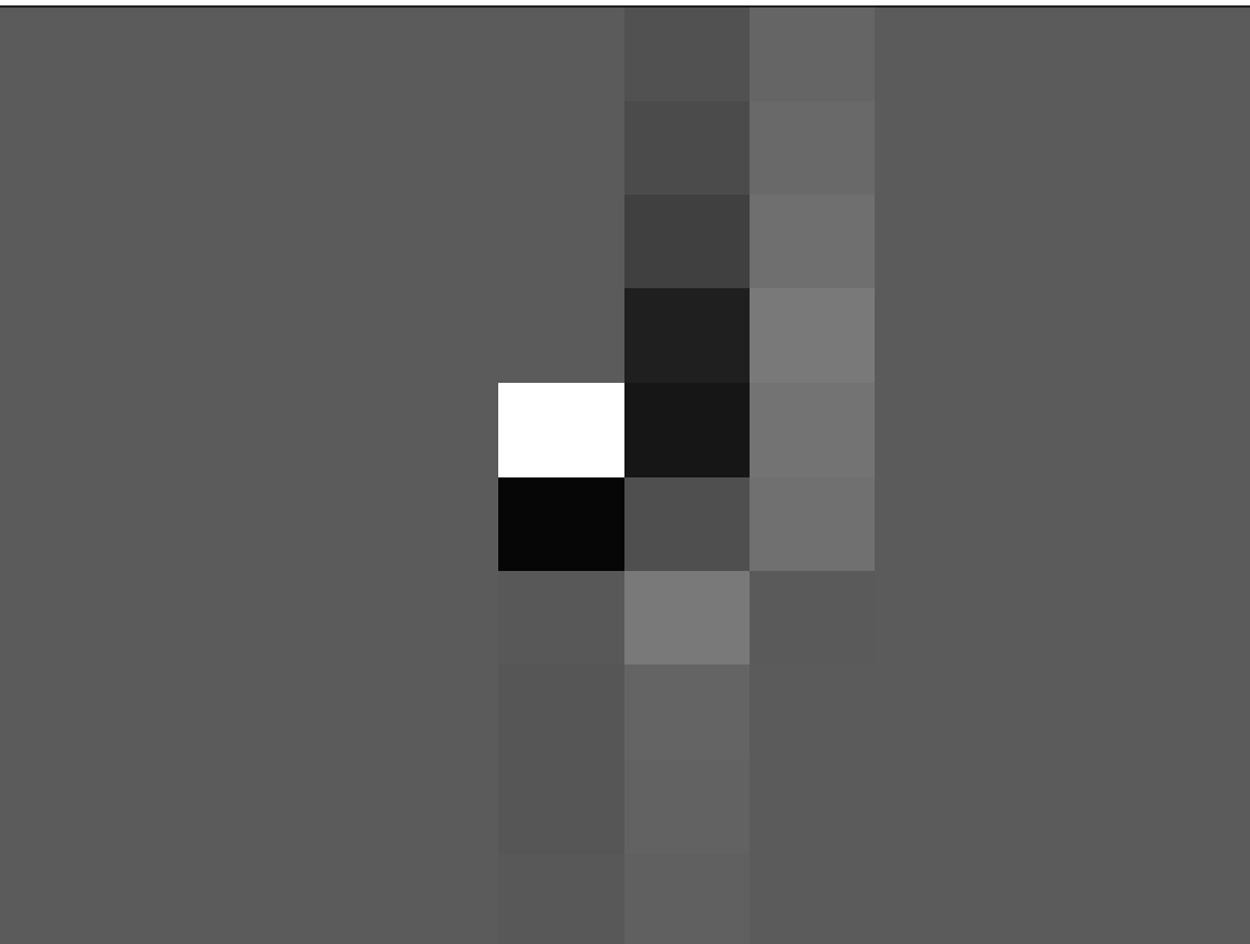
Wilson factor
