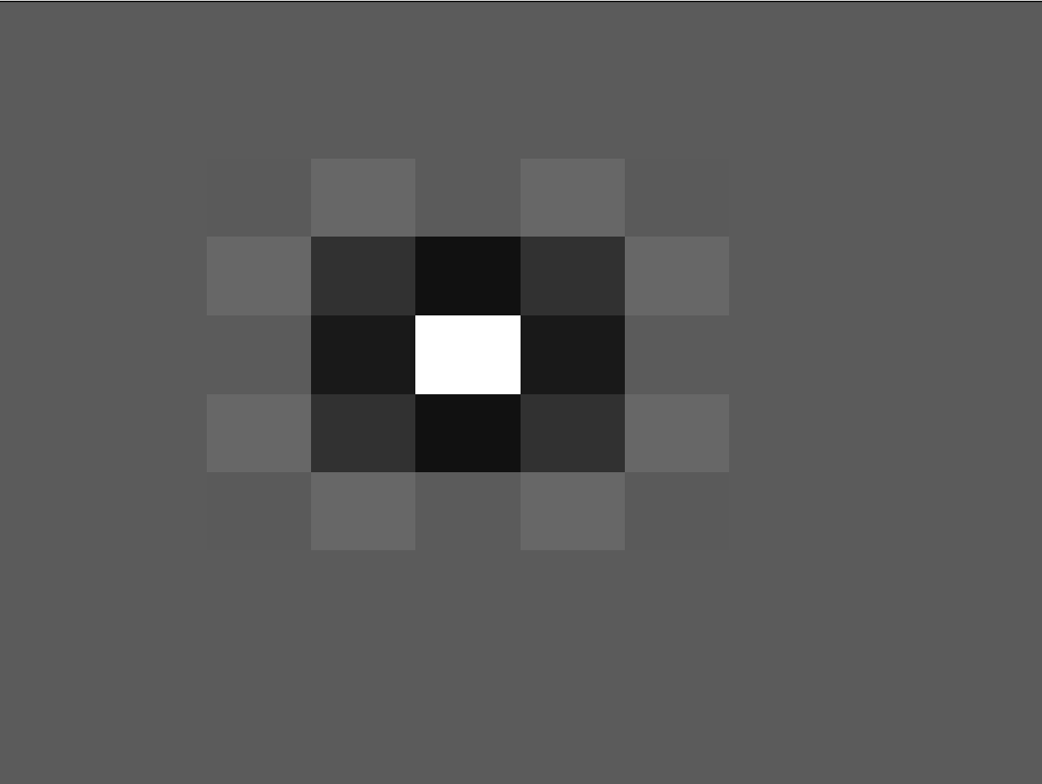
laplacian
