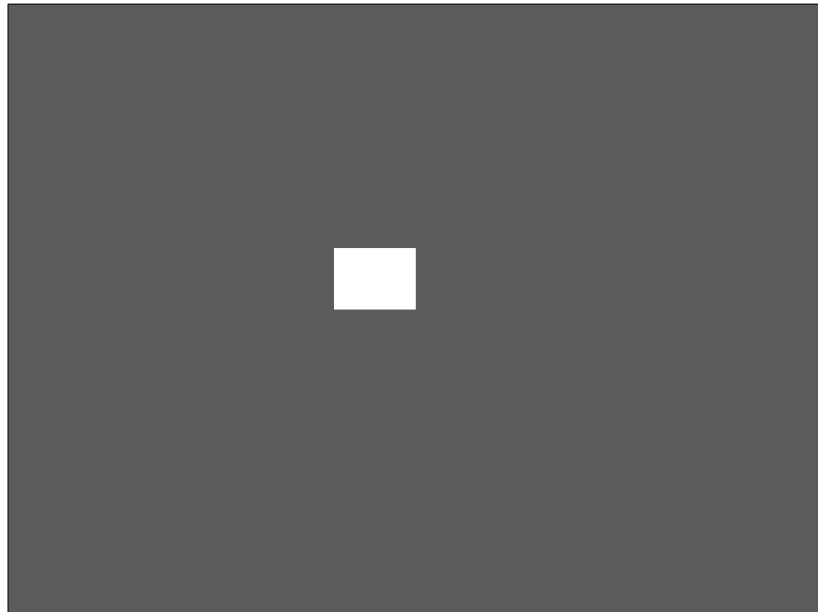
Wilson inversion
