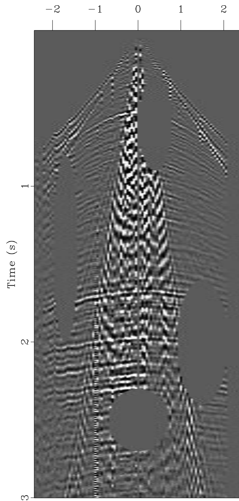
Shot Gather with Holes
