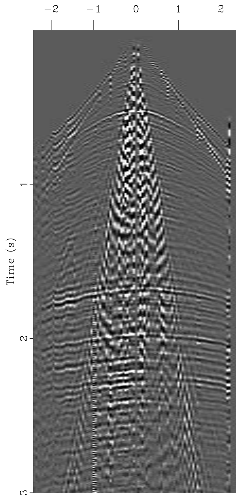
Shot Gather
