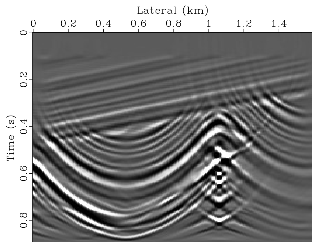
Migration0
