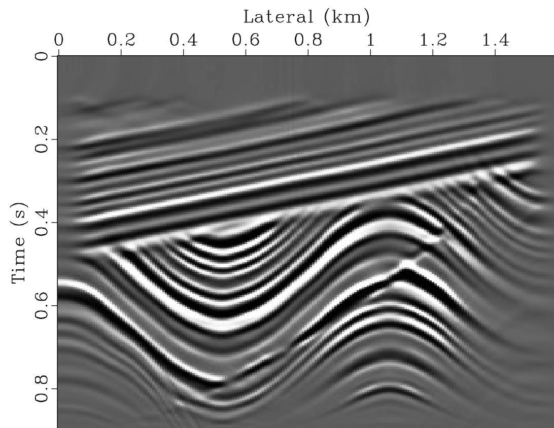
Velocity Continuation
