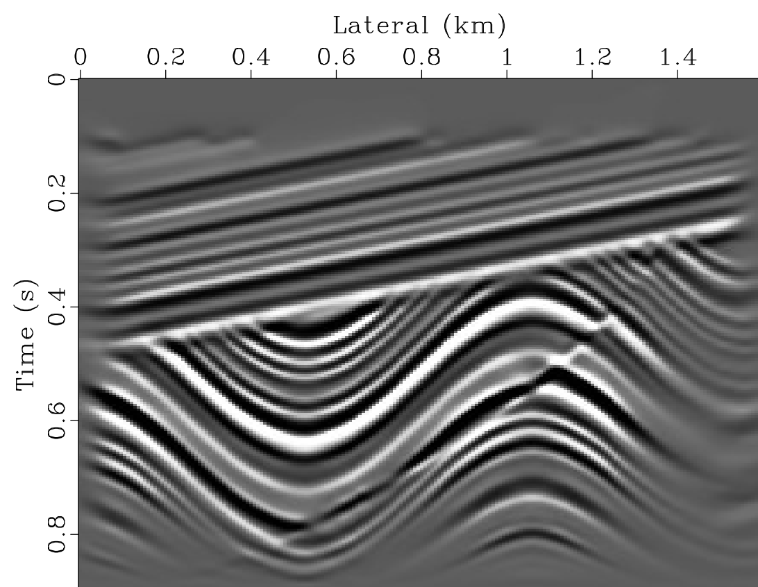
Migration1
