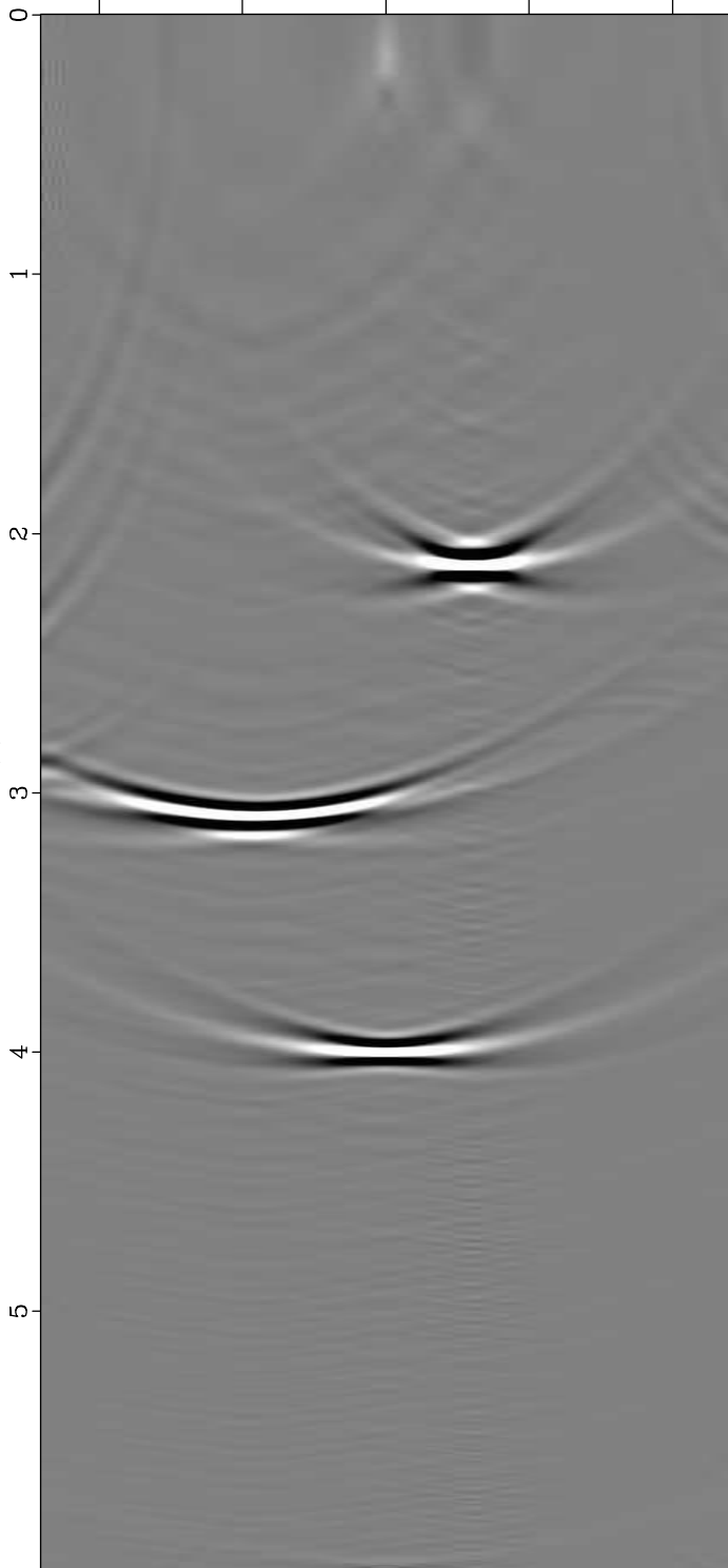
Dip Angle Gather ( x=0.25 km, v=0.75 km/s)
