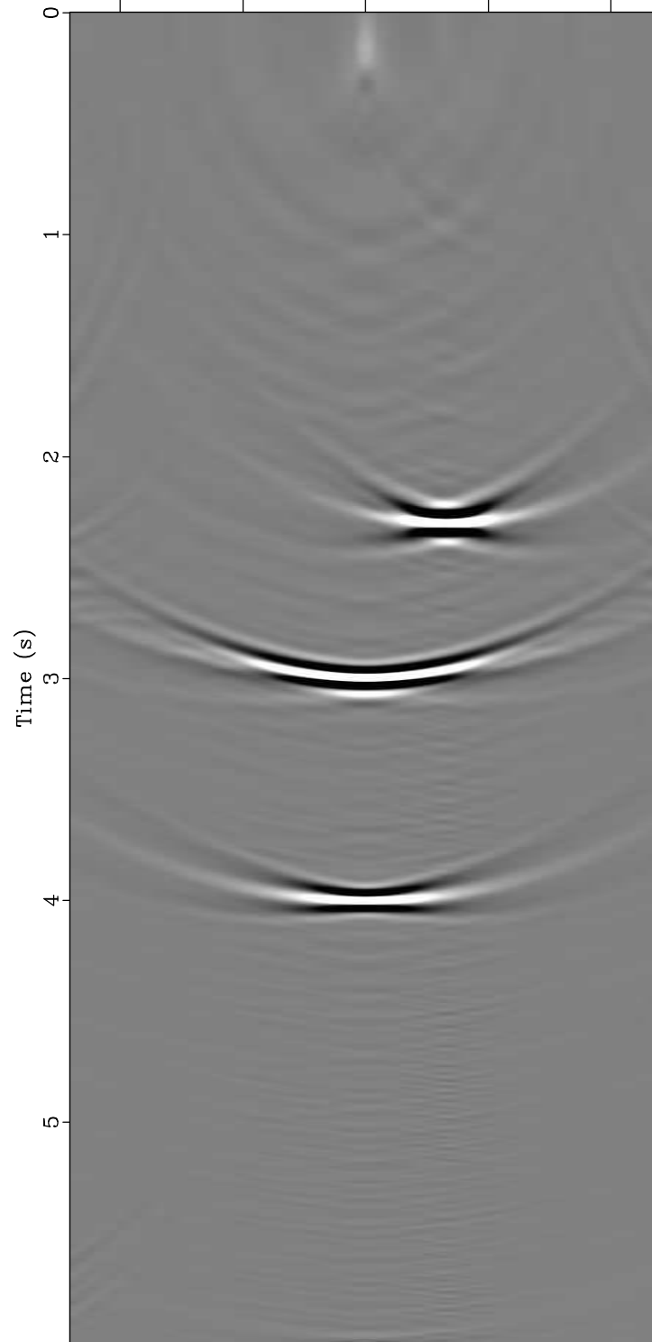
Dip Angle Gather ( x=0.5 km, v=0.75 km/s)
