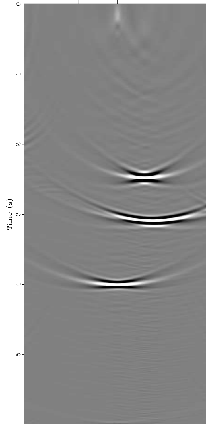
Dip Angle Gather ( x=0.75 km, v=0.75 km/s)
