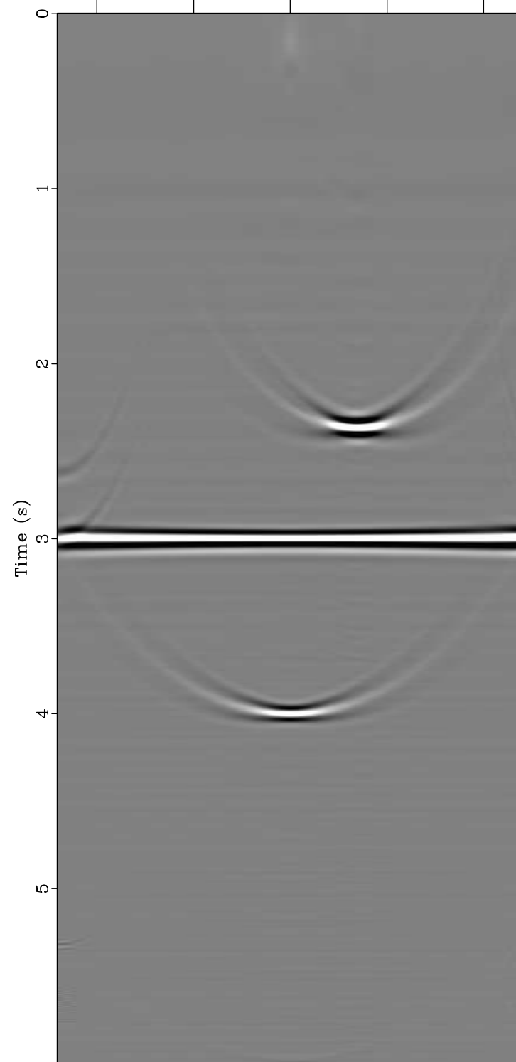
Dip Angle Gather ( x=0.5 km, v=1 km/s)
