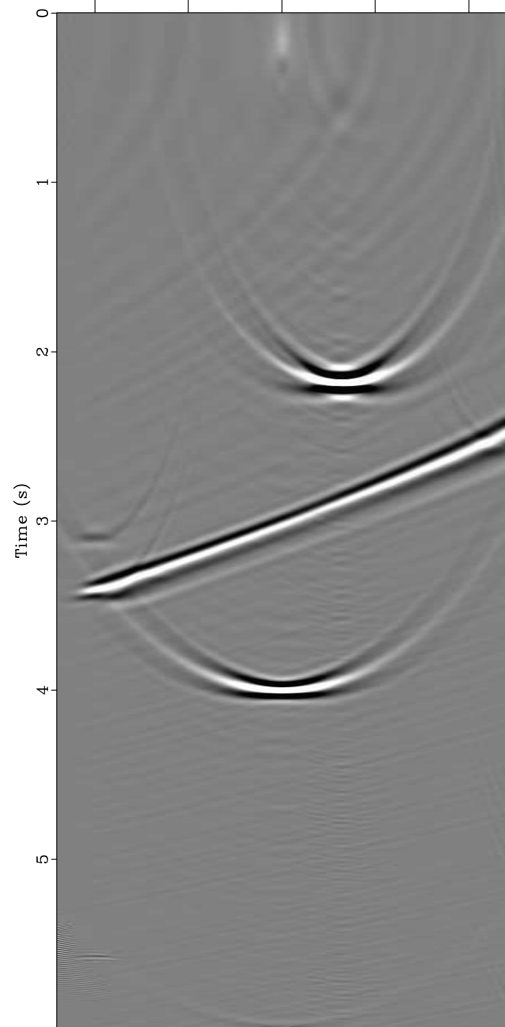
Dip Angle Gather ( x=0.25 km, v=1 km/s)
