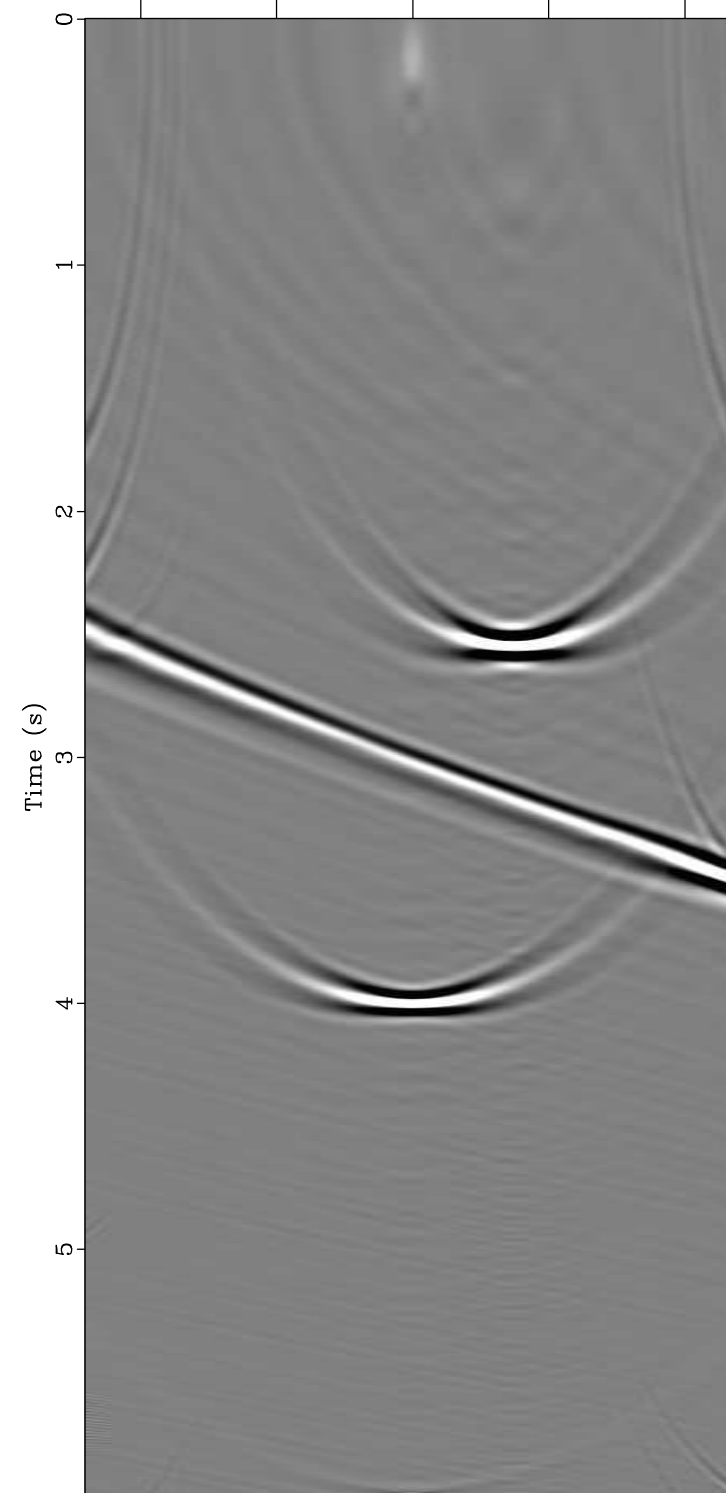
Dip Angle Gather ( x=0.75 km, v=1 km/s)
