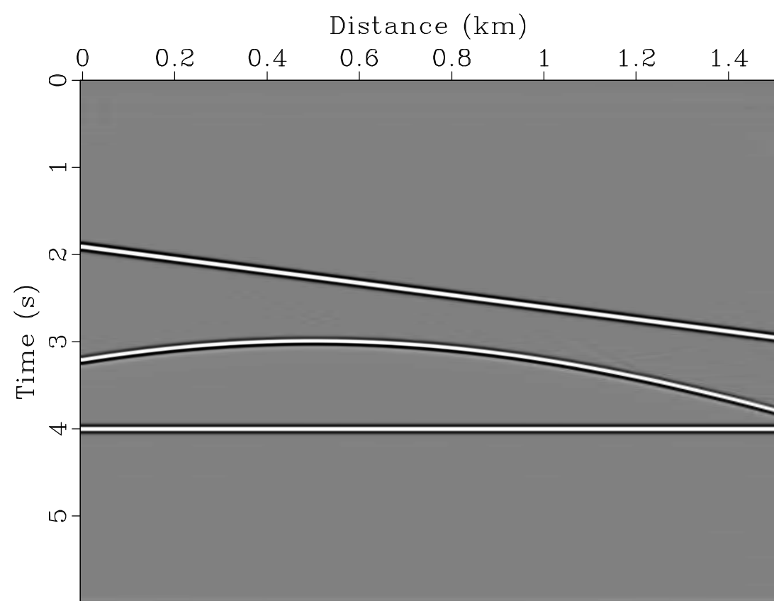
Velocity Continuation ( v=0.5 km/s)
