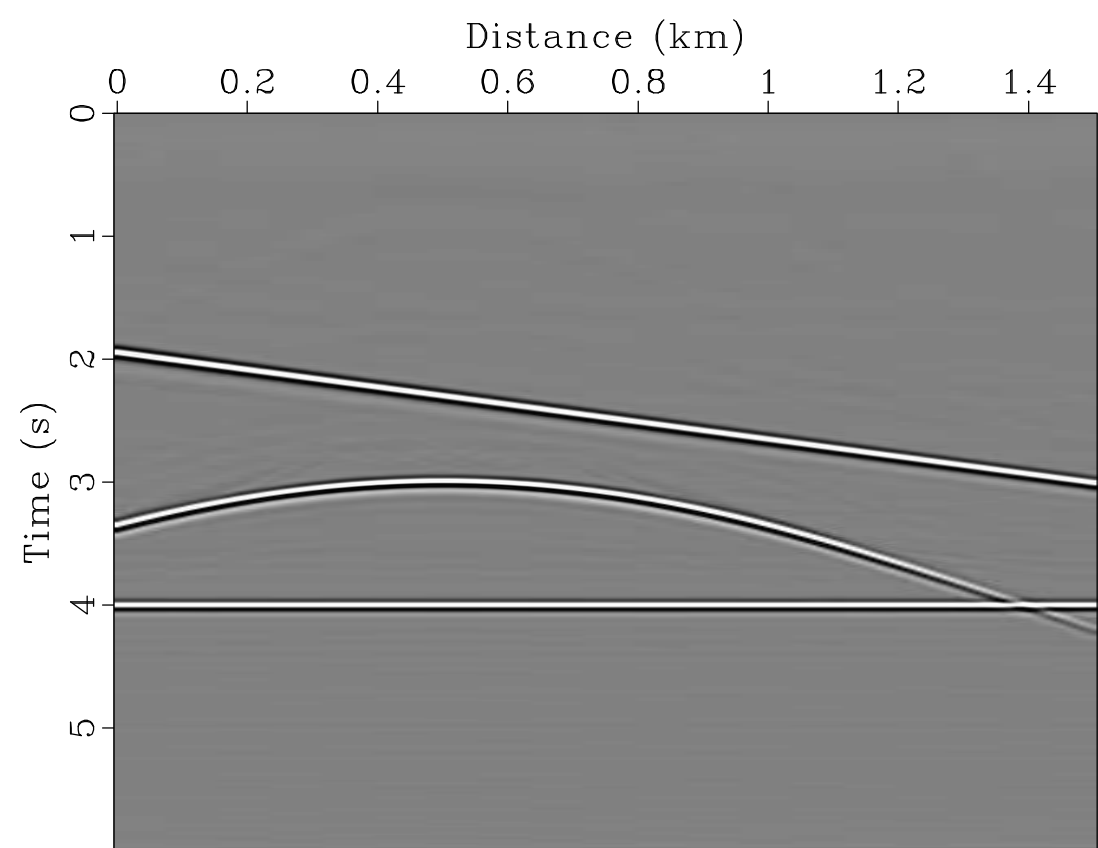
Velocity Continuation ( v=0.75 km/s)
