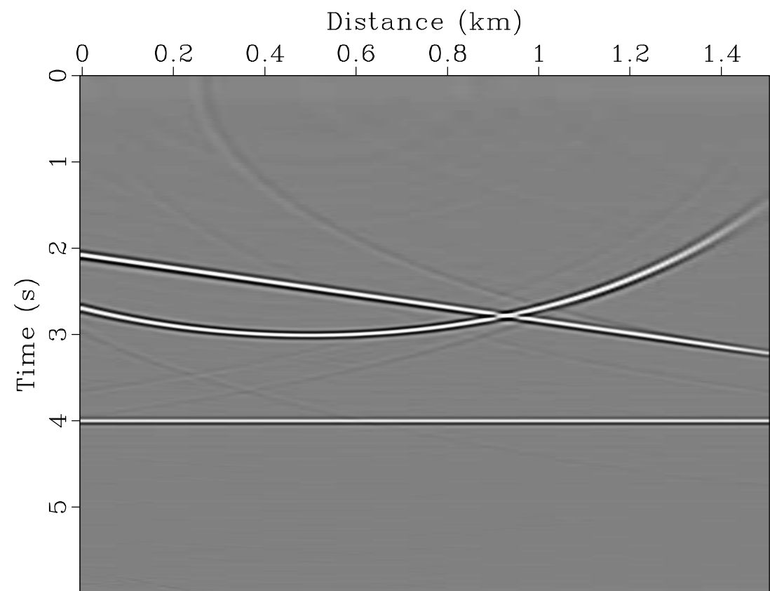
Velocity Continuation ( v=1.25 km/s)
