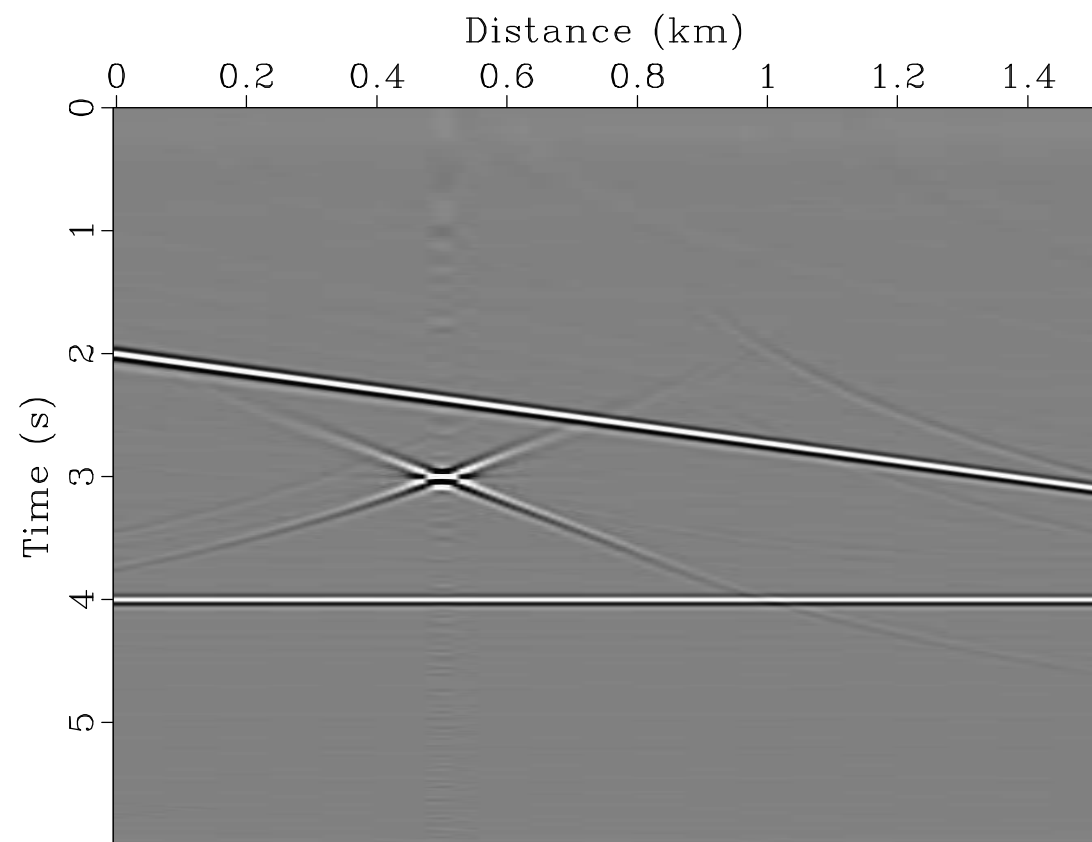
Velocity Continuation ( v=1 km/s)
