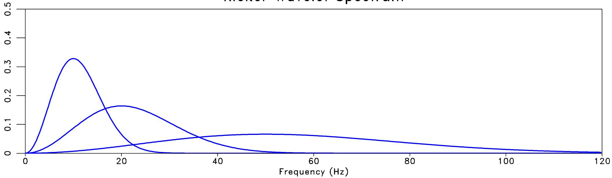
Ricker Wavelet Spectrum
