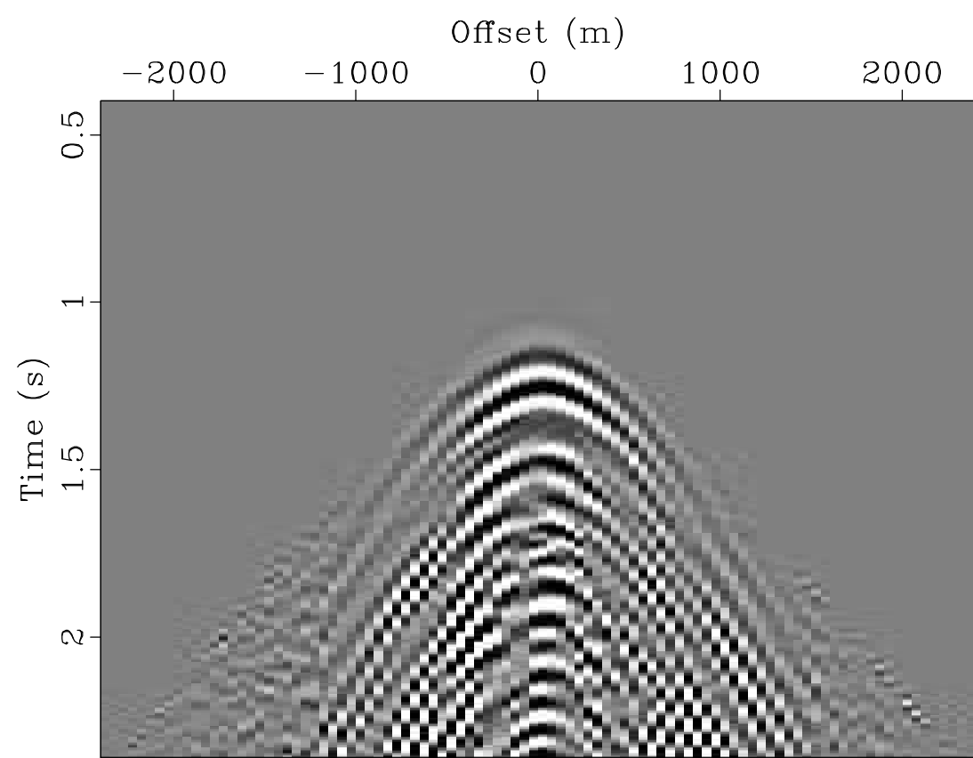
Estimated Noise
