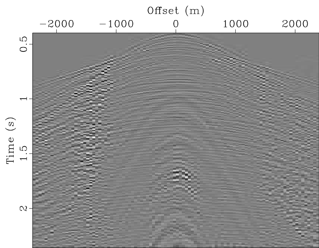
Estimated Signal
