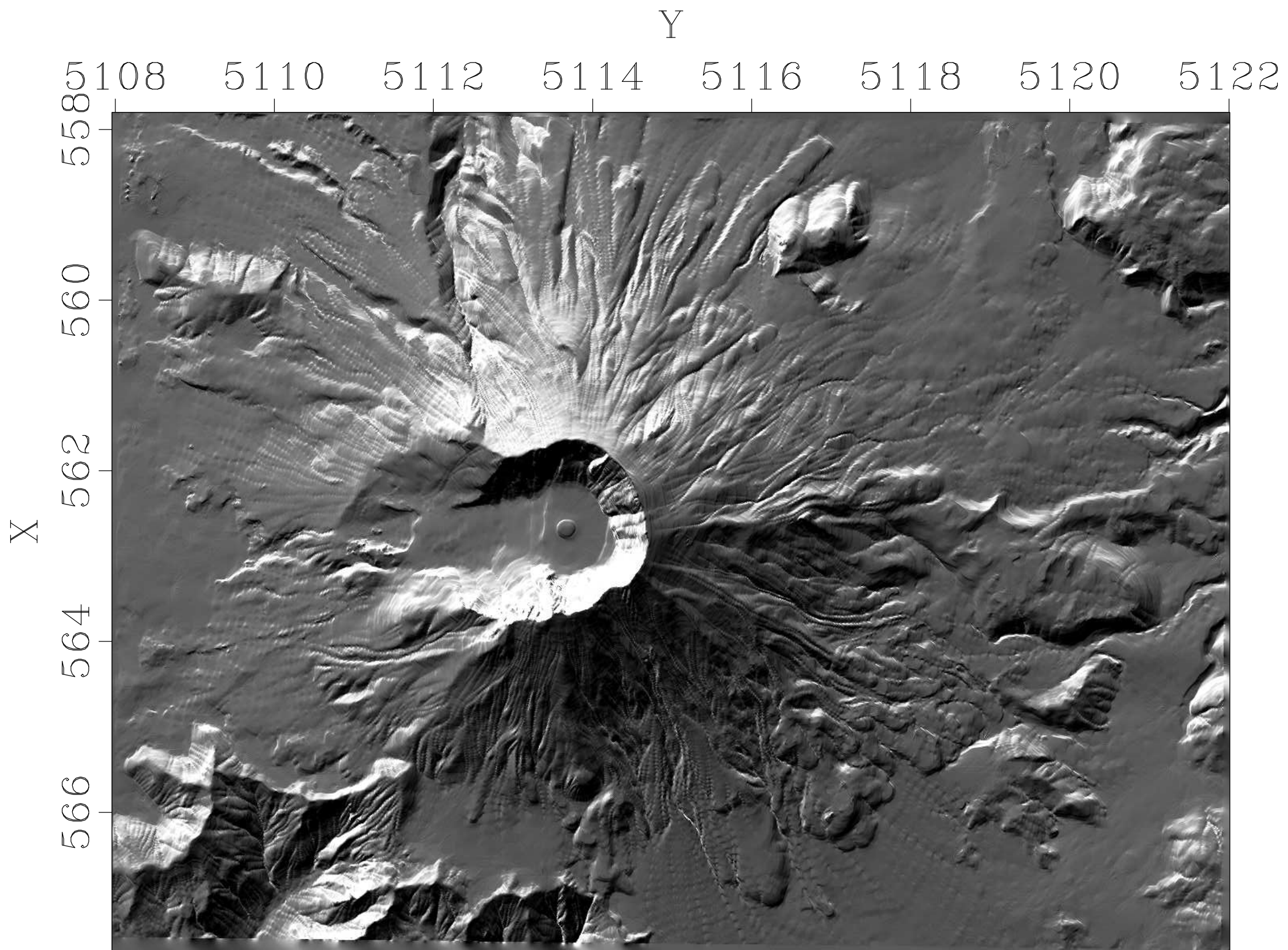
Directional Derivative at 30^\circ
