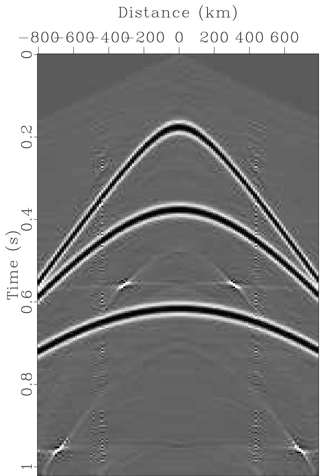
Remodelled cmp in LS sense
