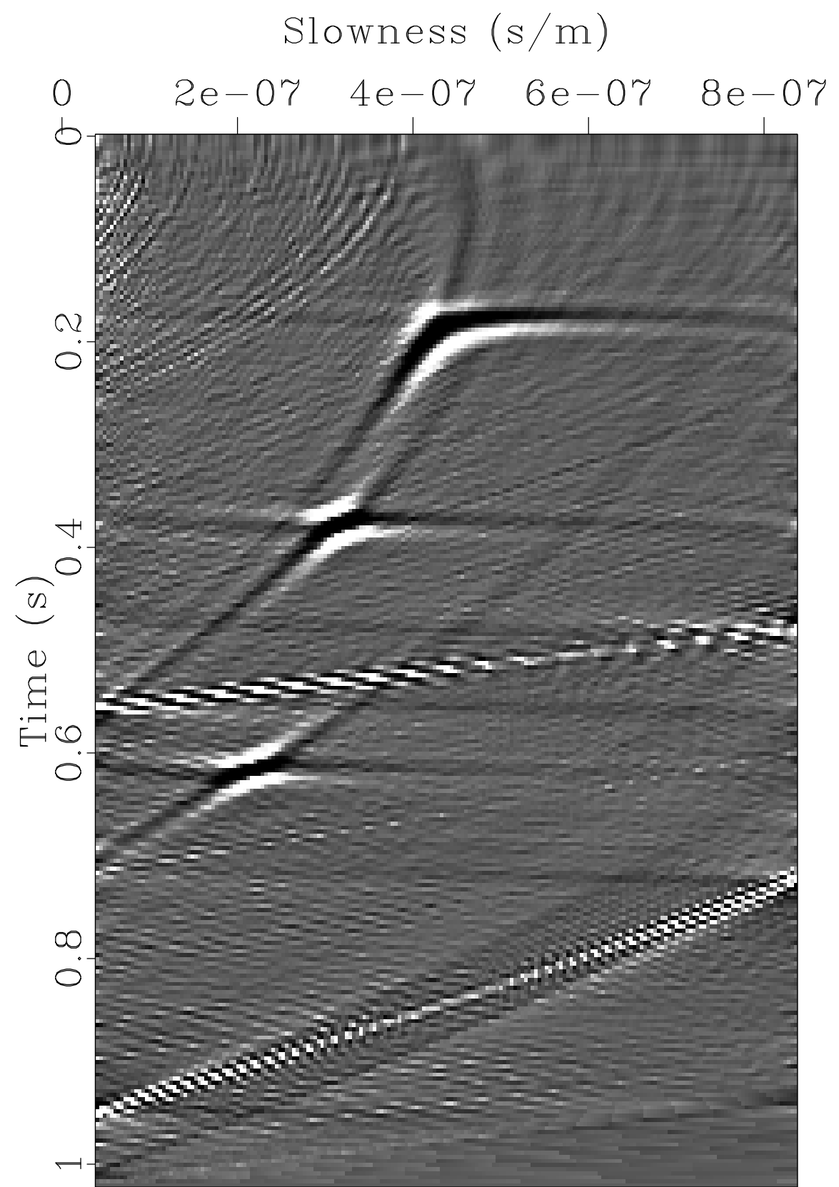
LS Velocity spectrum
