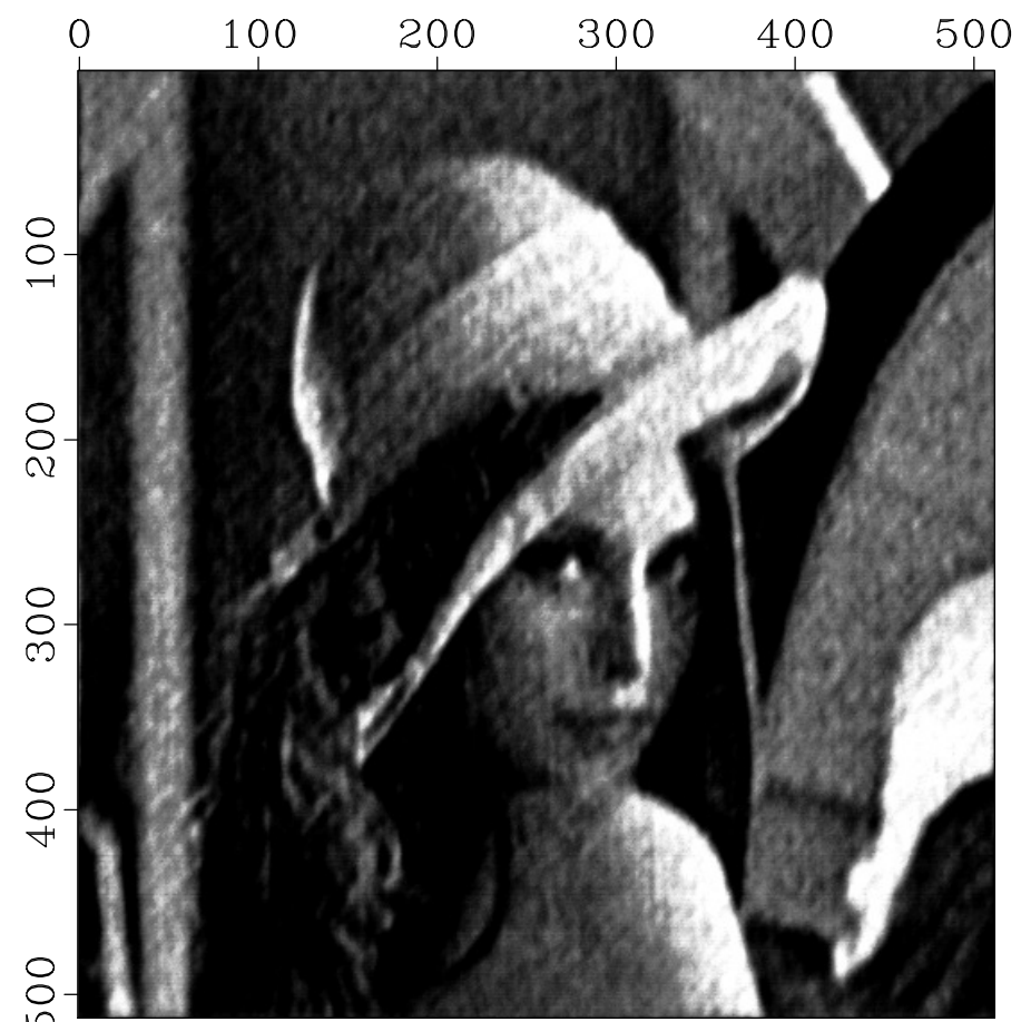
Thresholding in the Fourier domain
