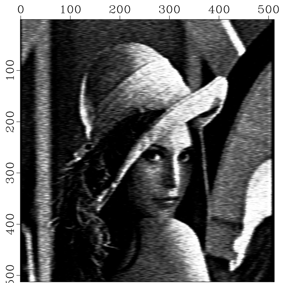
Noisy Lena LP filtered
