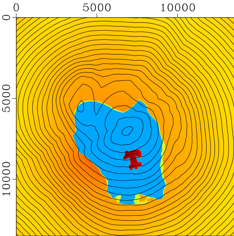
SEG/EAGE salt model
