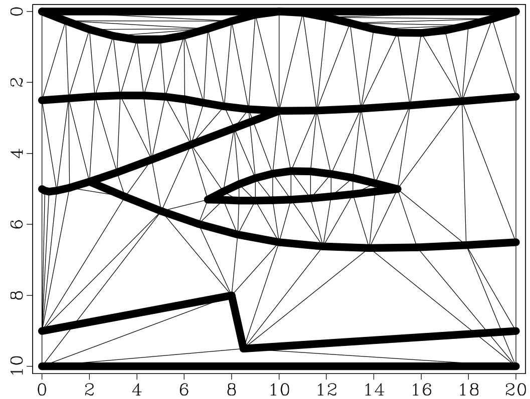
Nonconforming Triangulation
