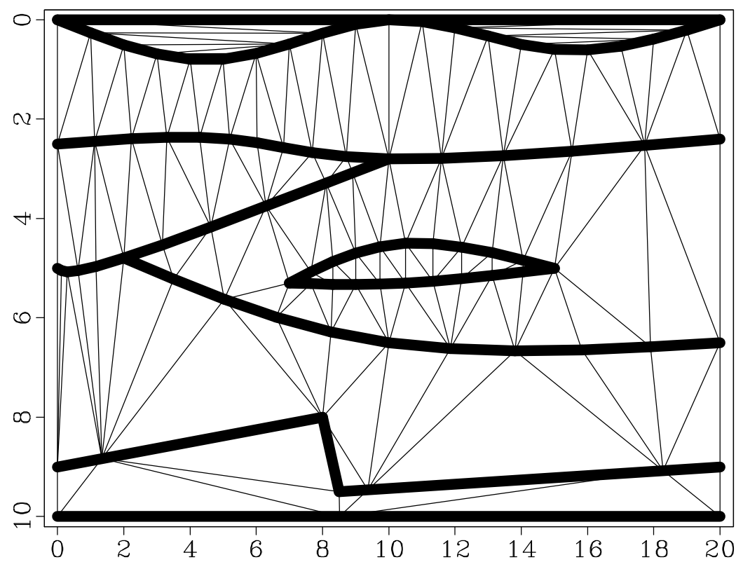
Conforming Triangulation
