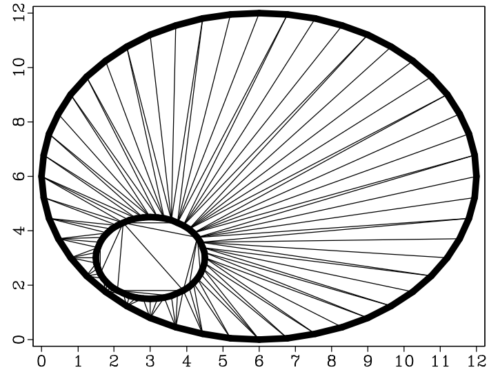
Delaunay Triangulation
