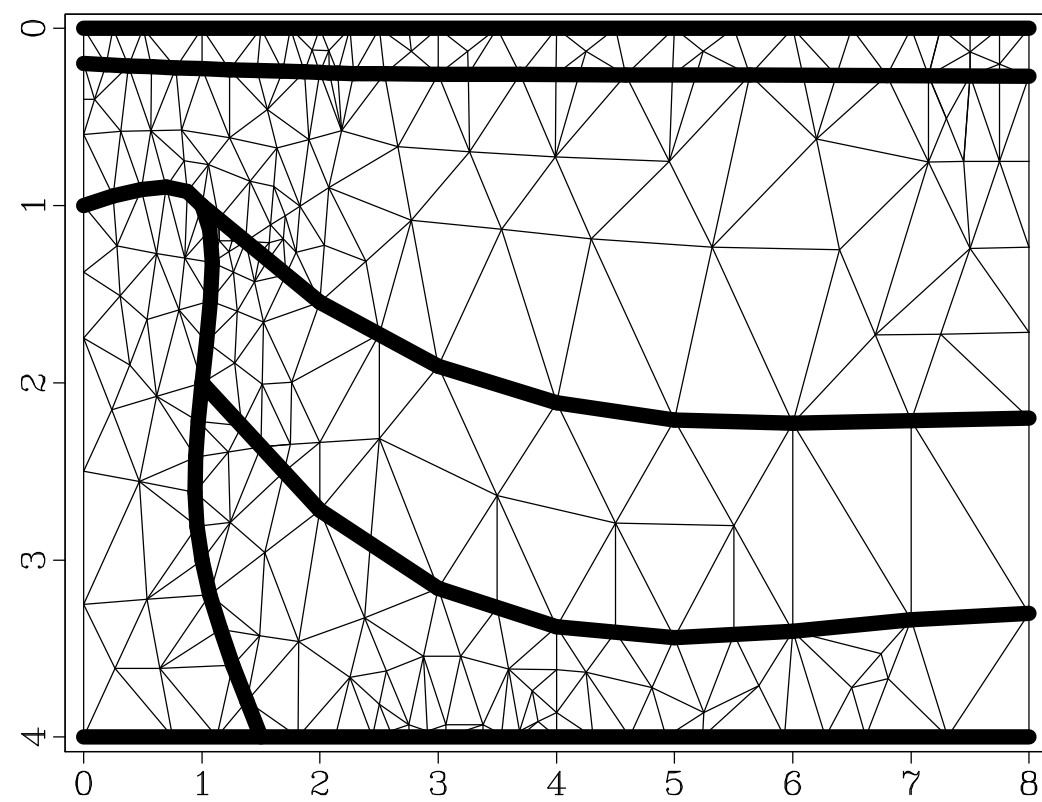
Refinement
