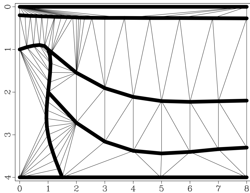
Conforming Triangulation
