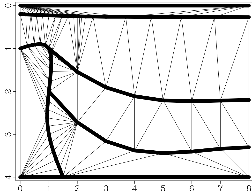
Nonconforming Triangulation
