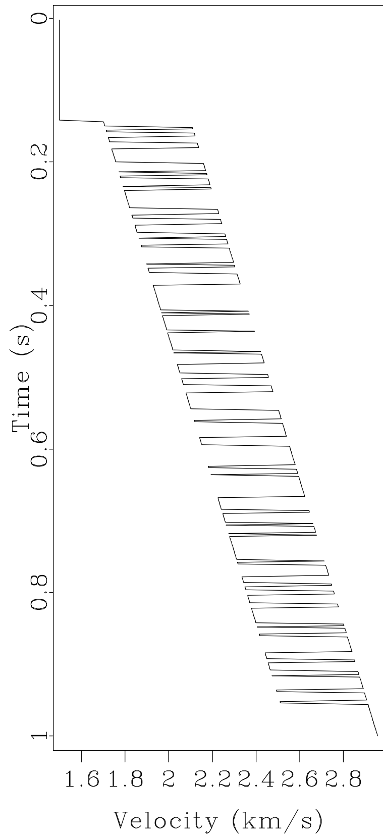
Interval Velocity
