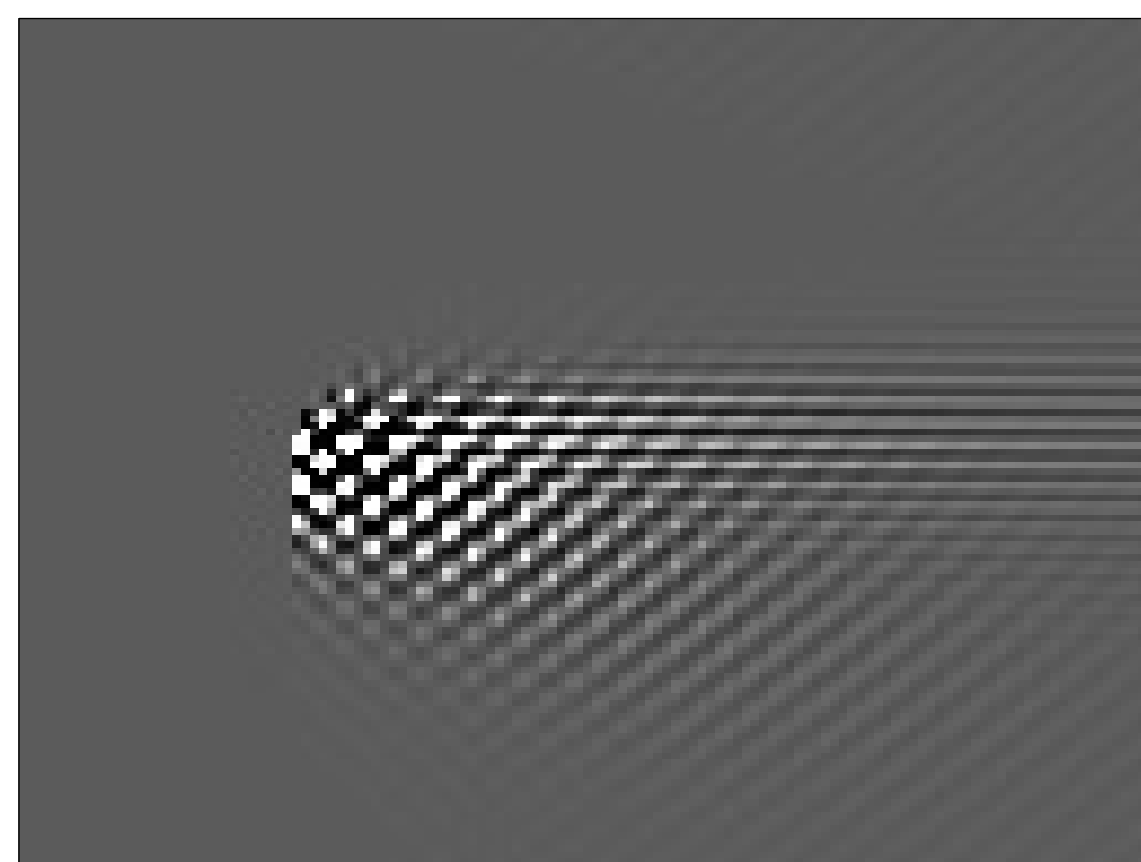
spike/PEF
