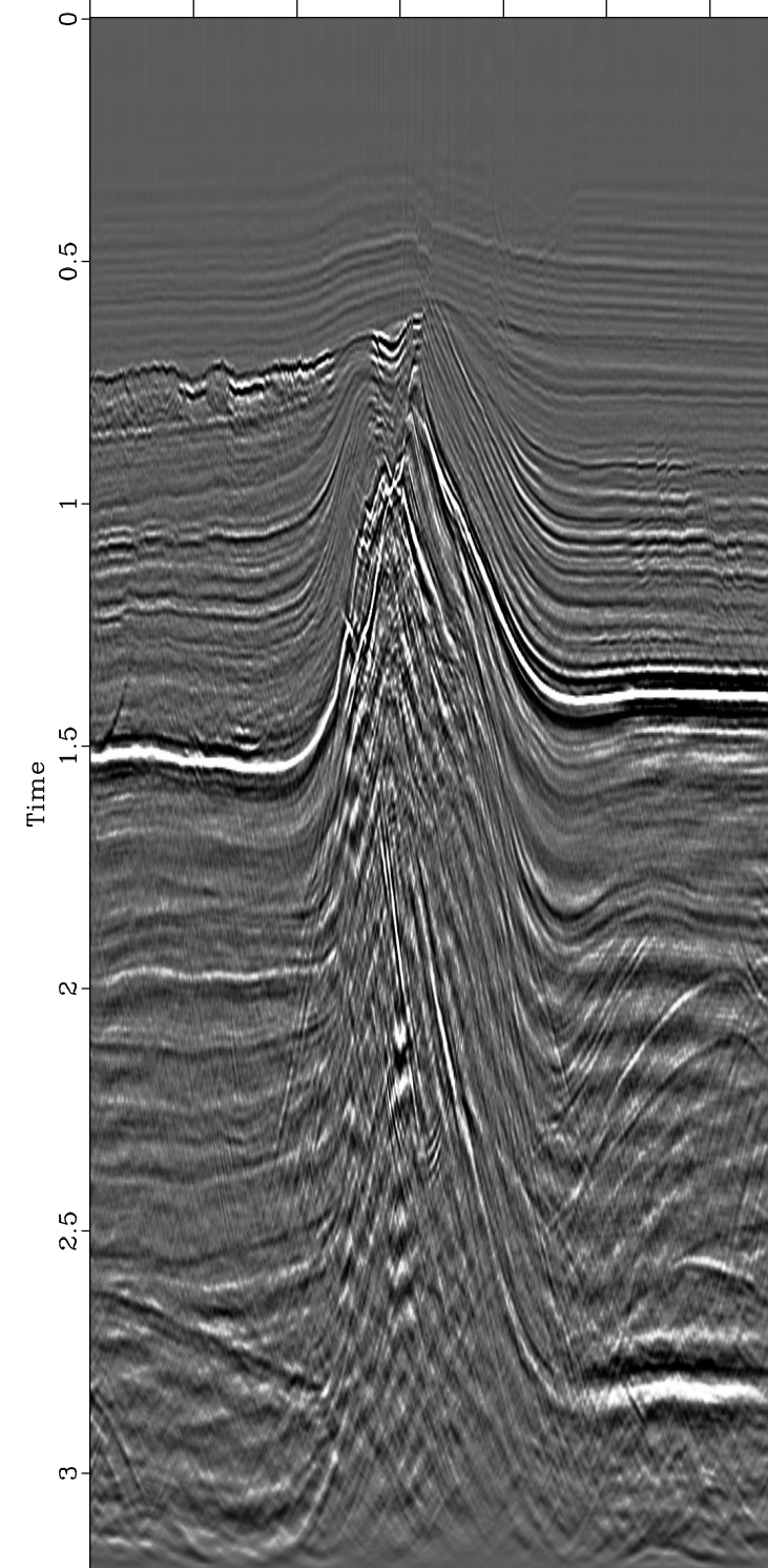
Velocity Continuation 0 -> 1
