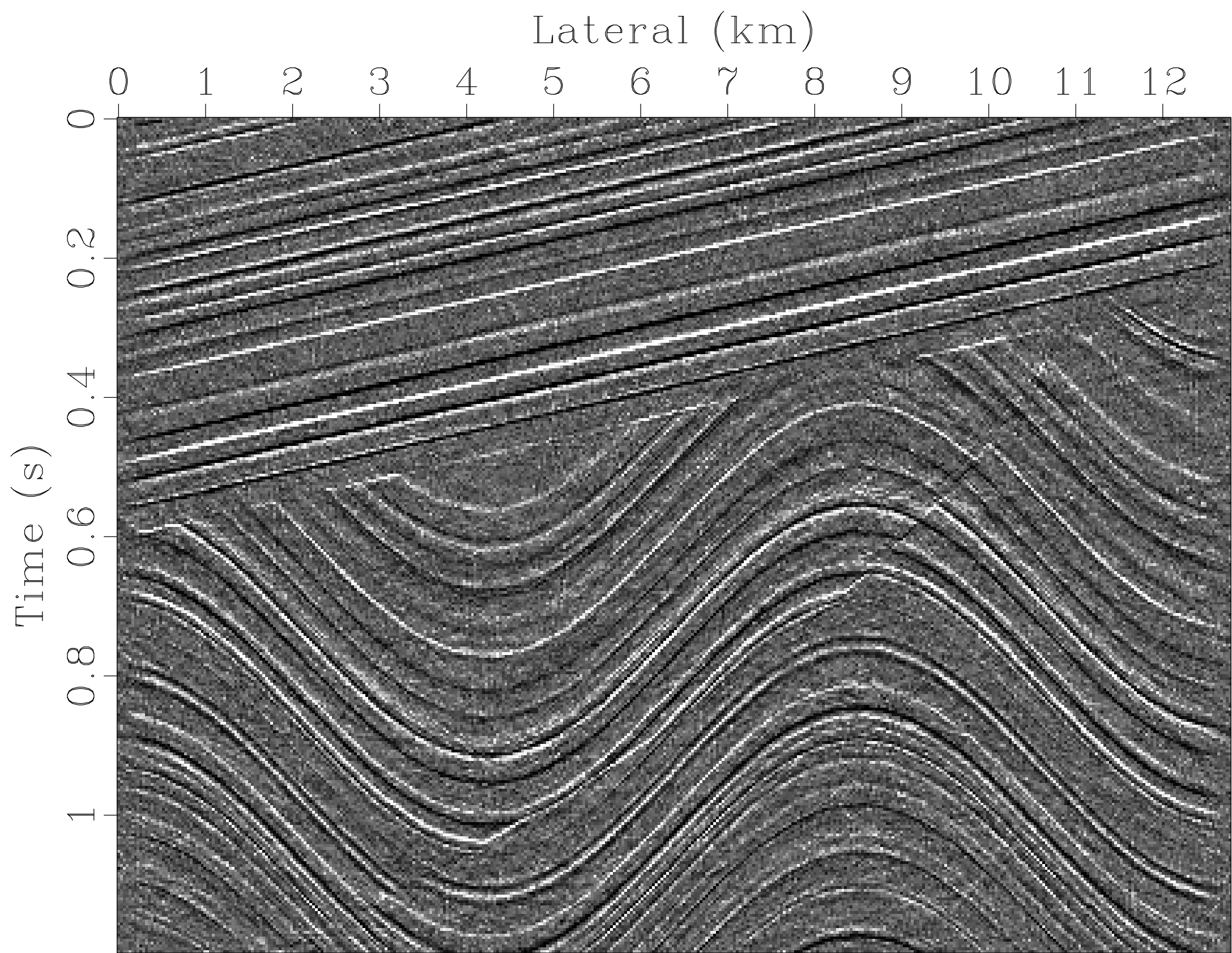
Denoised image
