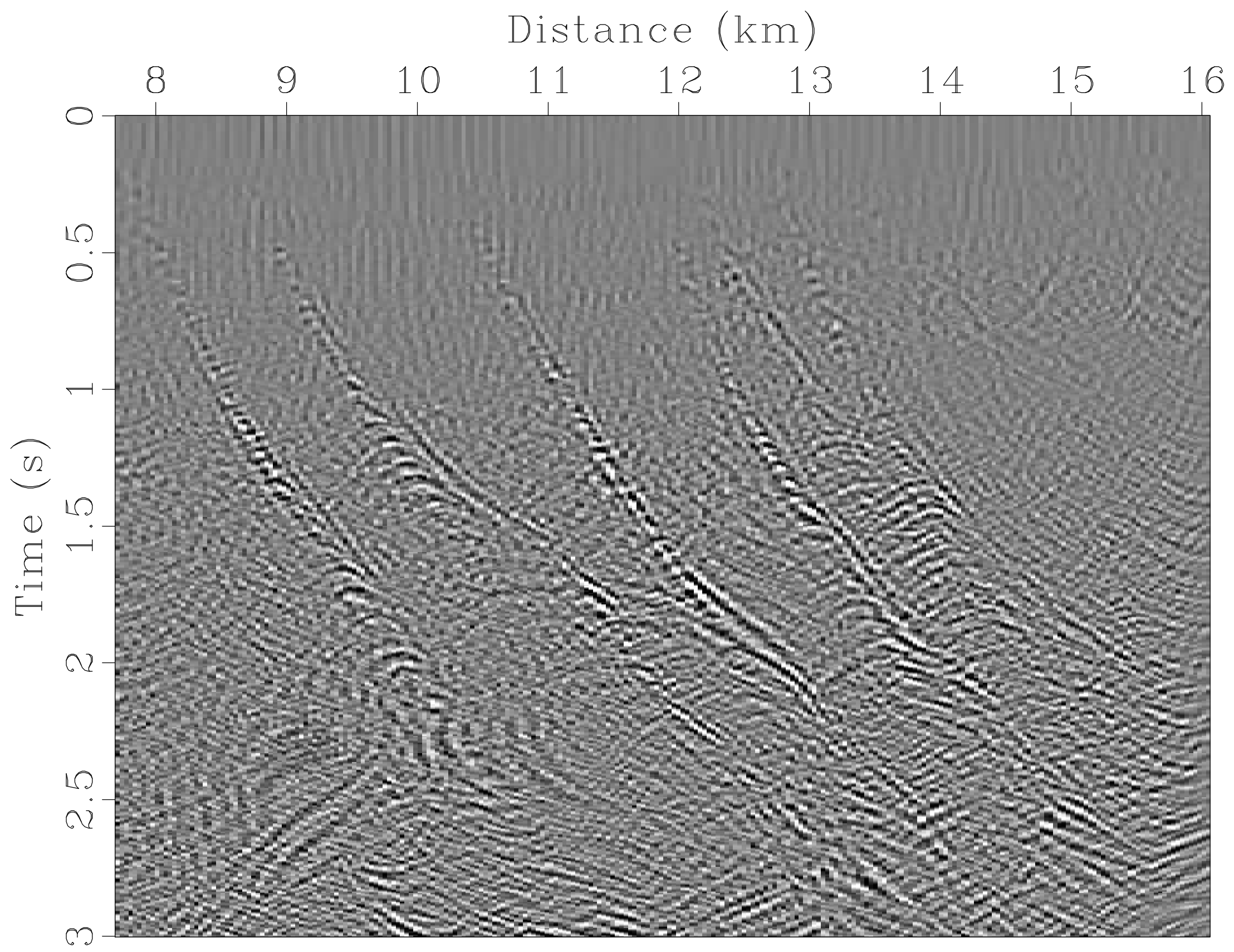
Migrated Diffractions
