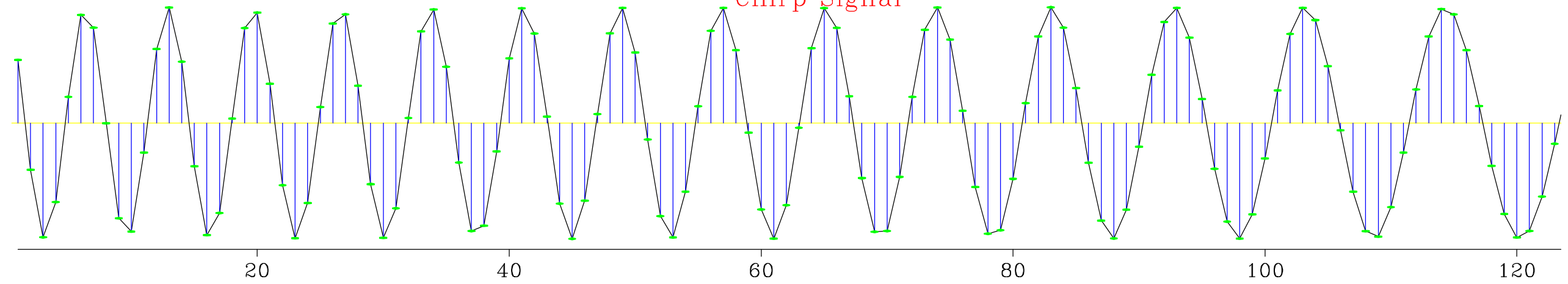
1-D Wavelet Transform
